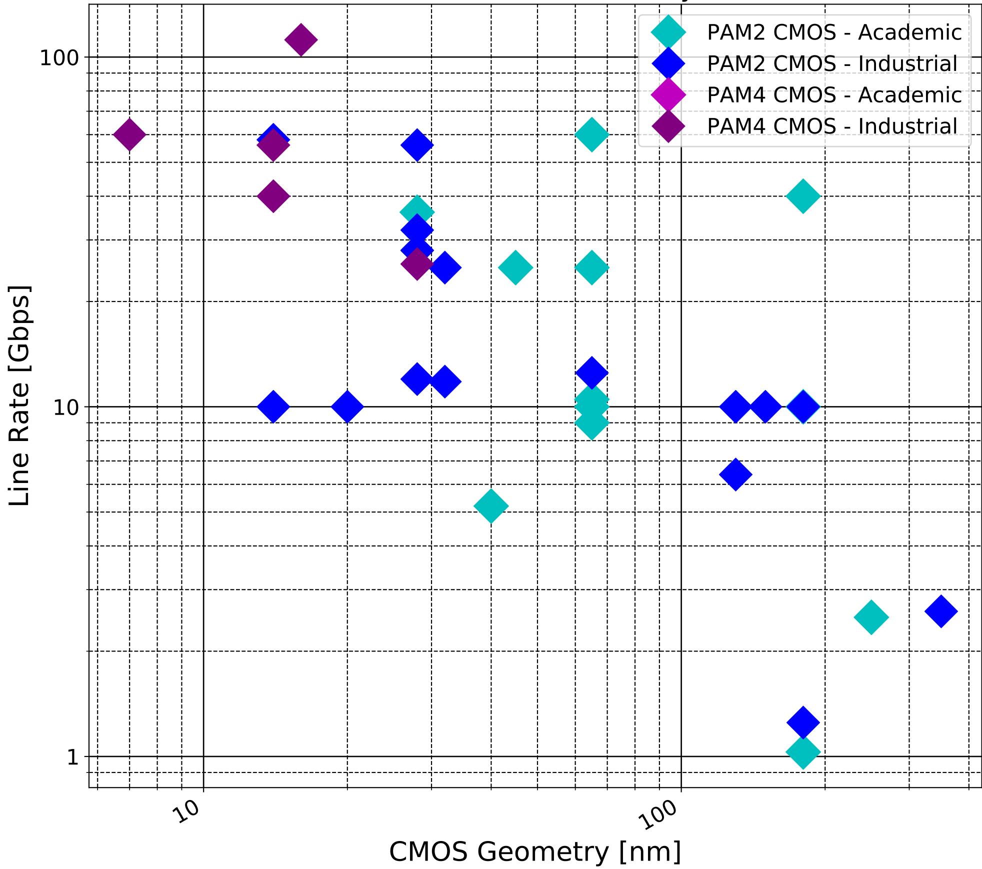
Line Rate vs CMOS Geometry [nm]
